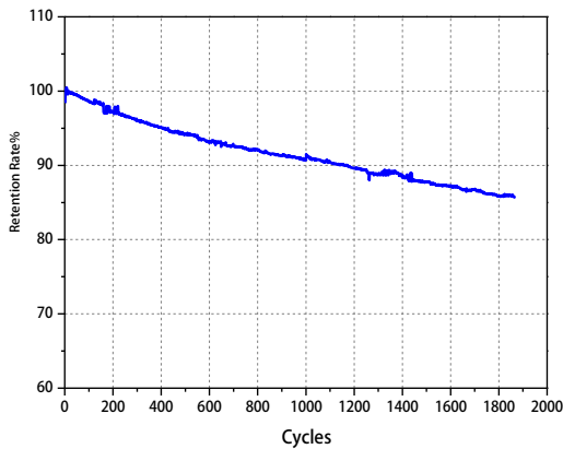
Cycles & Capacity Retention Rate, 0.2C
